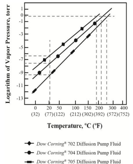
Figure 1: Vapor Pressure
